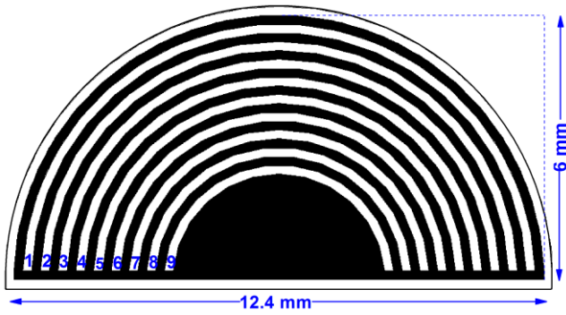
Fig. 1: 9-bit chipless RFID tag.
