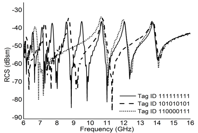
Fig. 7: Different tag IDs for Tag 4.
