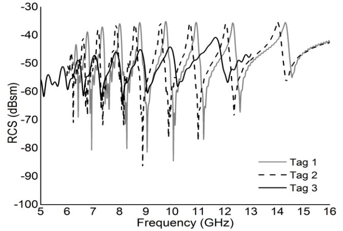
Fig. 3: Comparison of three proposed tags using different substrates.
