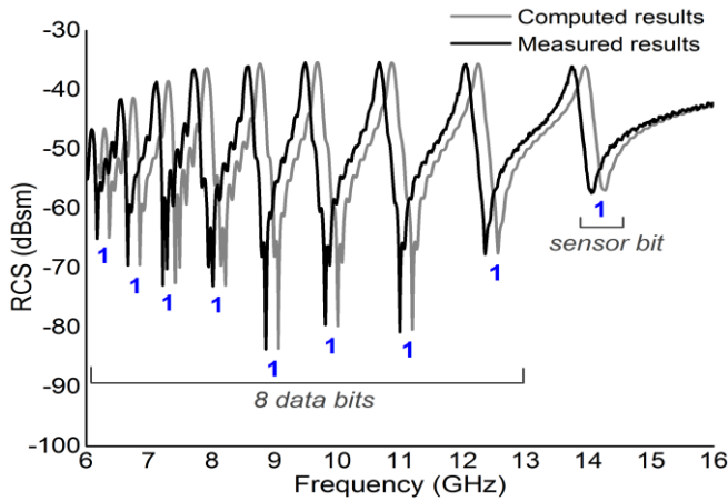
Fig. 4: RCS response of Tag 4.
