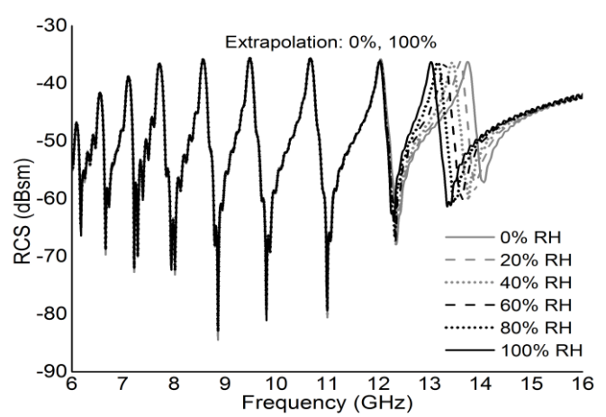
Fig. 6: Humidity sensing behavior of Tag 4.
