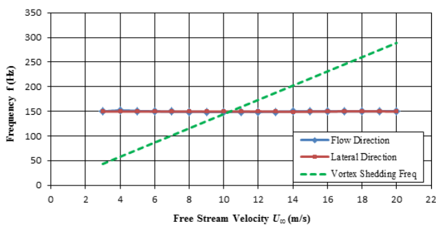
Fig. 8: Observed frequency response.
