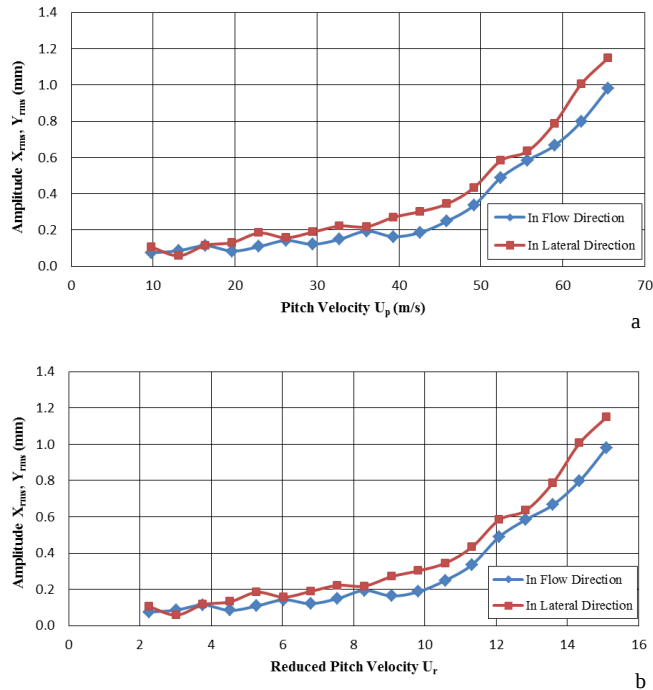
Fig. 10: Vibration amplitude response of target tube (a) with pitch velocity (b) with reduced pitch velocity.
