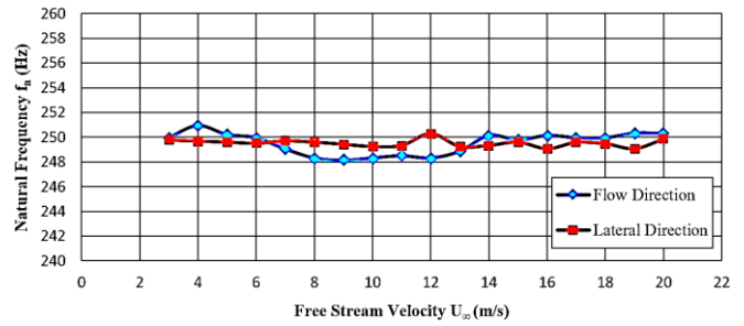
Fig. 5: Natural (Response) frequency plot of the target tube.
