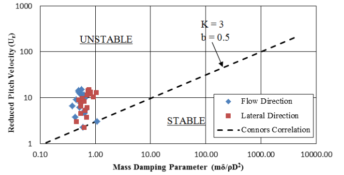
Fig. 14: Plot of mass-damping parameter Vs reduced velocity (stability map).
