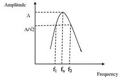
Fig. 12: Bode's plot for damping [9].
