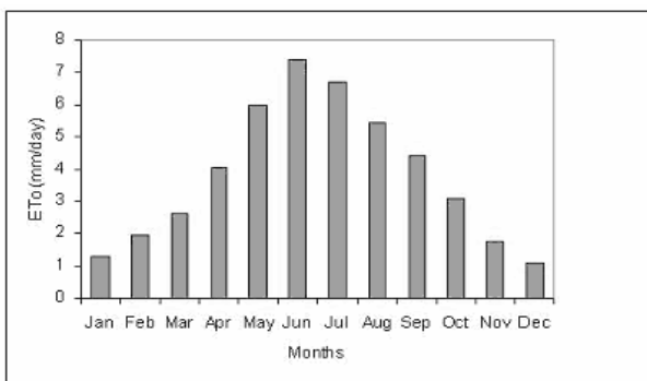
Figure 1. Measured daily ET_o from class A pan (1984-2008)
