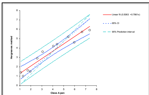
Figure 2. Comparison between daily average Potential evapotranspiration estimated by Hergreaves method with class A pan.
