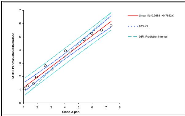
Figure 4. Comparison between Daily average Potential evapotranspiration estimated by FAO56 Penman-Monteith method with class A pan
