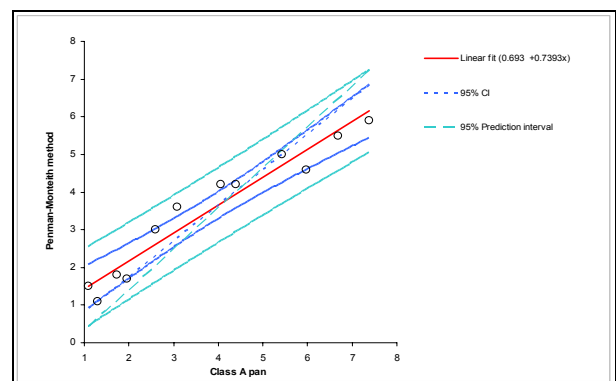
Figure 3. Comparison between daily average Potential evapotranspiration estimated by Penman-Monteith method with class A pan
