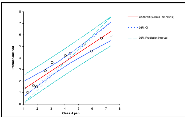
Figure 5. Comparison between daily average Potential evapotranspiration estimated by Penman method with class A pan.
